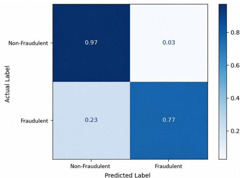
Figure 3. Confusion Matrix for the Best-Performing Supervised Model: Logistic Regression
