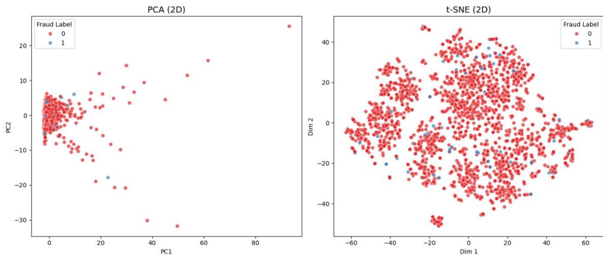
Figure 2. Comparison of Potential-Fraud and Non-Fraud Observations in Two-Dimensional PCA and t-SNE Space Before and After Data Balancing
