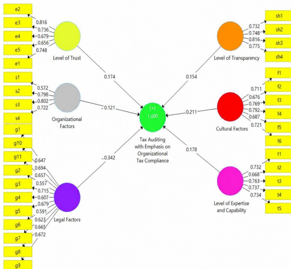
Figure 1. Model with Factor Loading Coefficients
